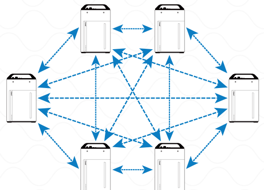
Hybrid Networking
