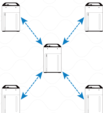
Star Networking
