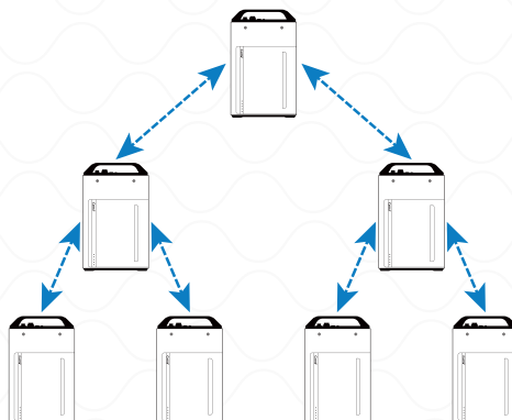
Tree Networking
